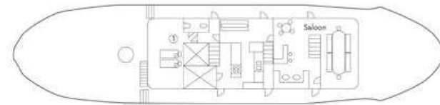
Main Deck
